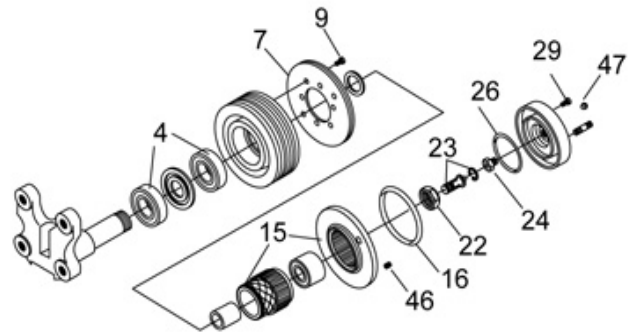
HT/S Advantage Fan Drive (split ring design)
