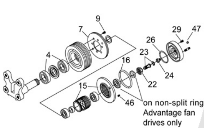
HT/S Advantage Fan Drive (original design)
